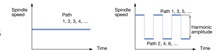
<Normal threading>
