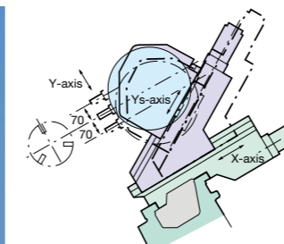
X•Y plane Radial Y-axis machining examples
